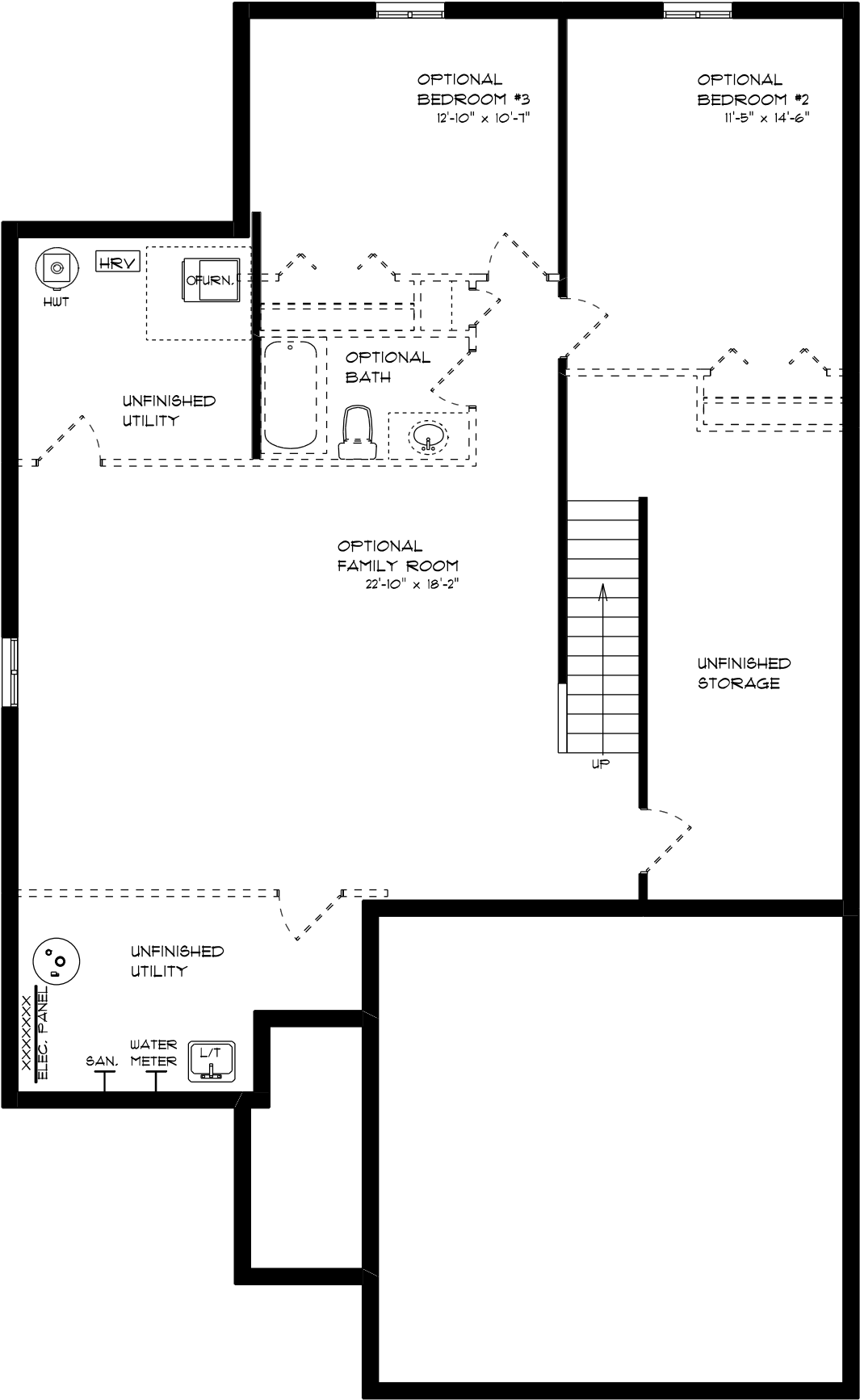
FOUNDATION PLAN 920 SQ.FT. OPTIONAL FINISHED
