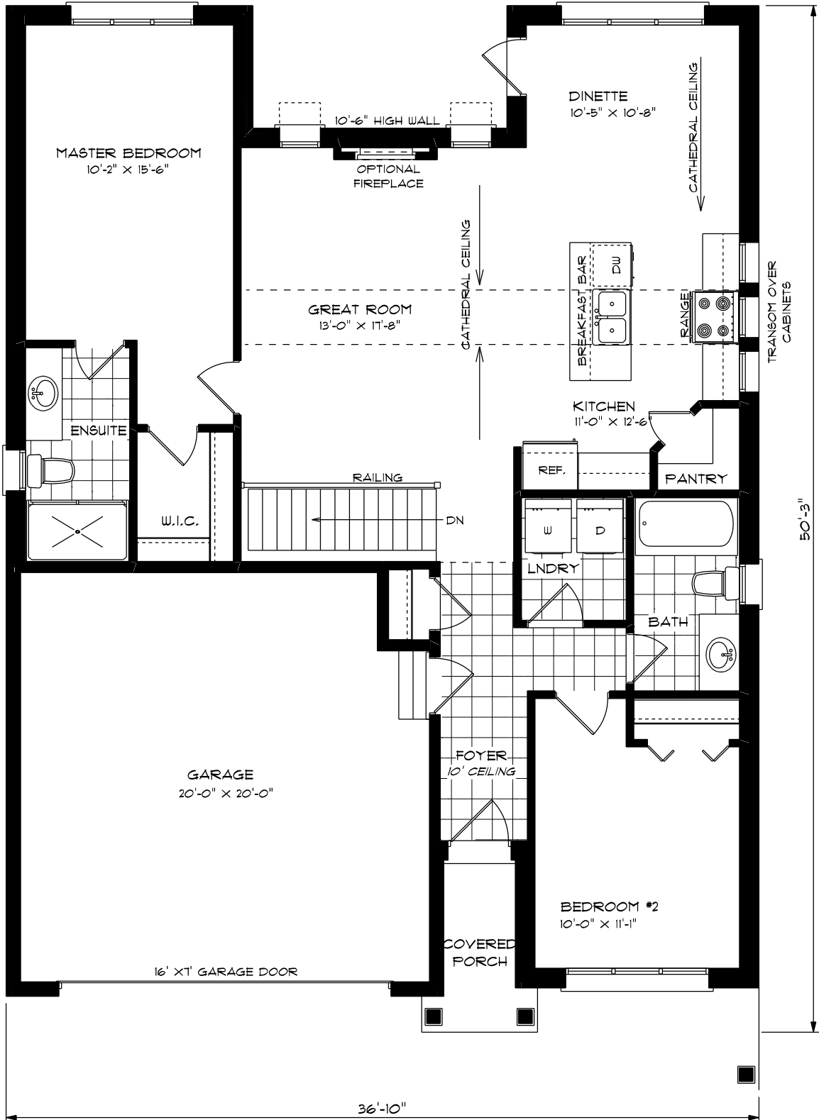
MAIN FLOOR PLAN 1251 SQ.FT.
