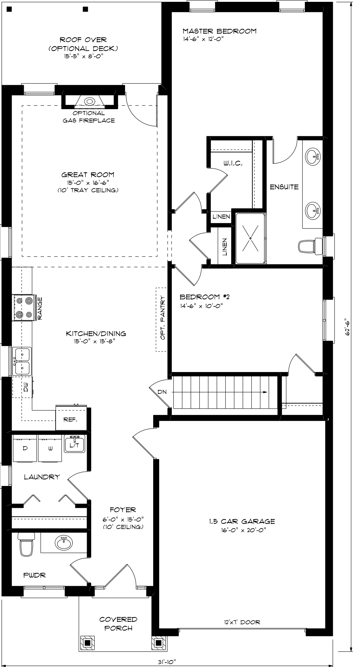
MAIN FLOOR PLAN 'C'
