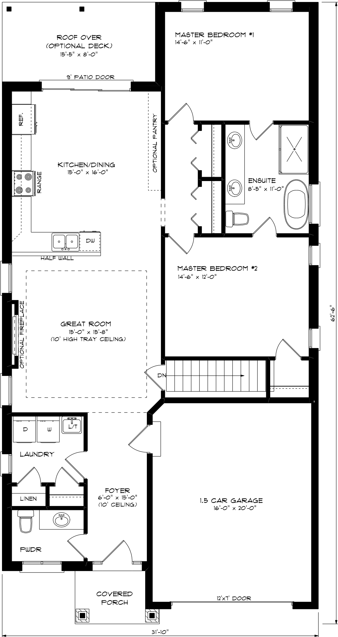
MAIN FLOOR PLAN 'A' 1415 SQ.FT.
