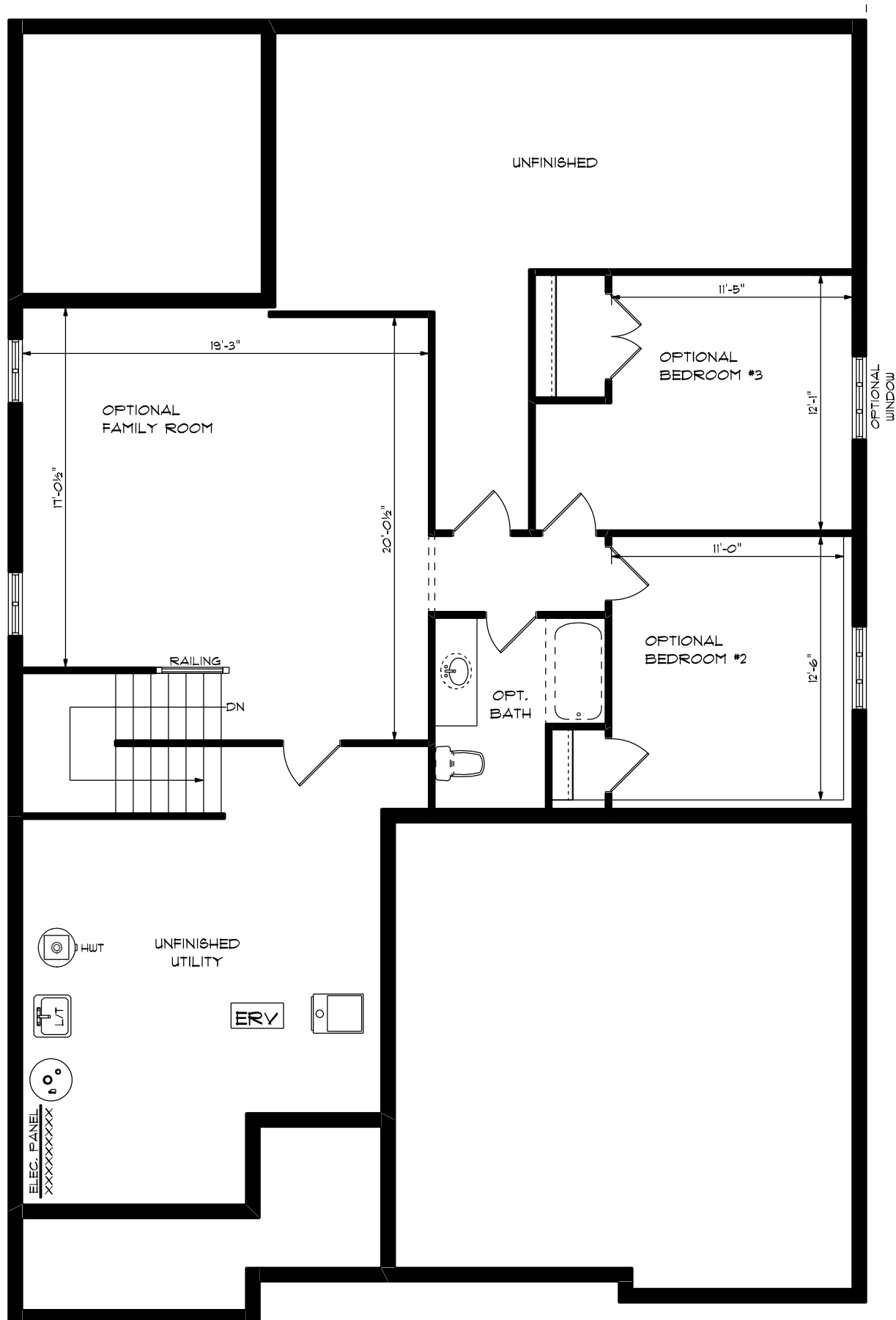
FOUNDATION PLAN OPTIONAL FINISHED AREA: 826 SQ.FT.
