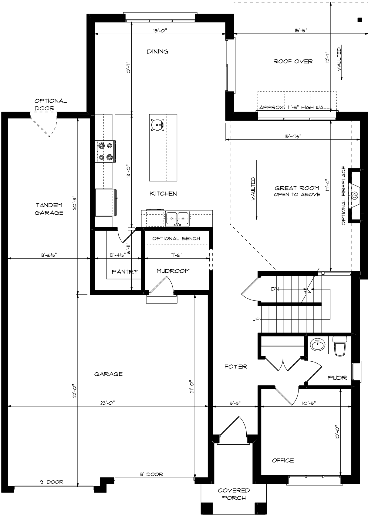
MAIN FLOOR PLAN 1226 SQ.FT.
