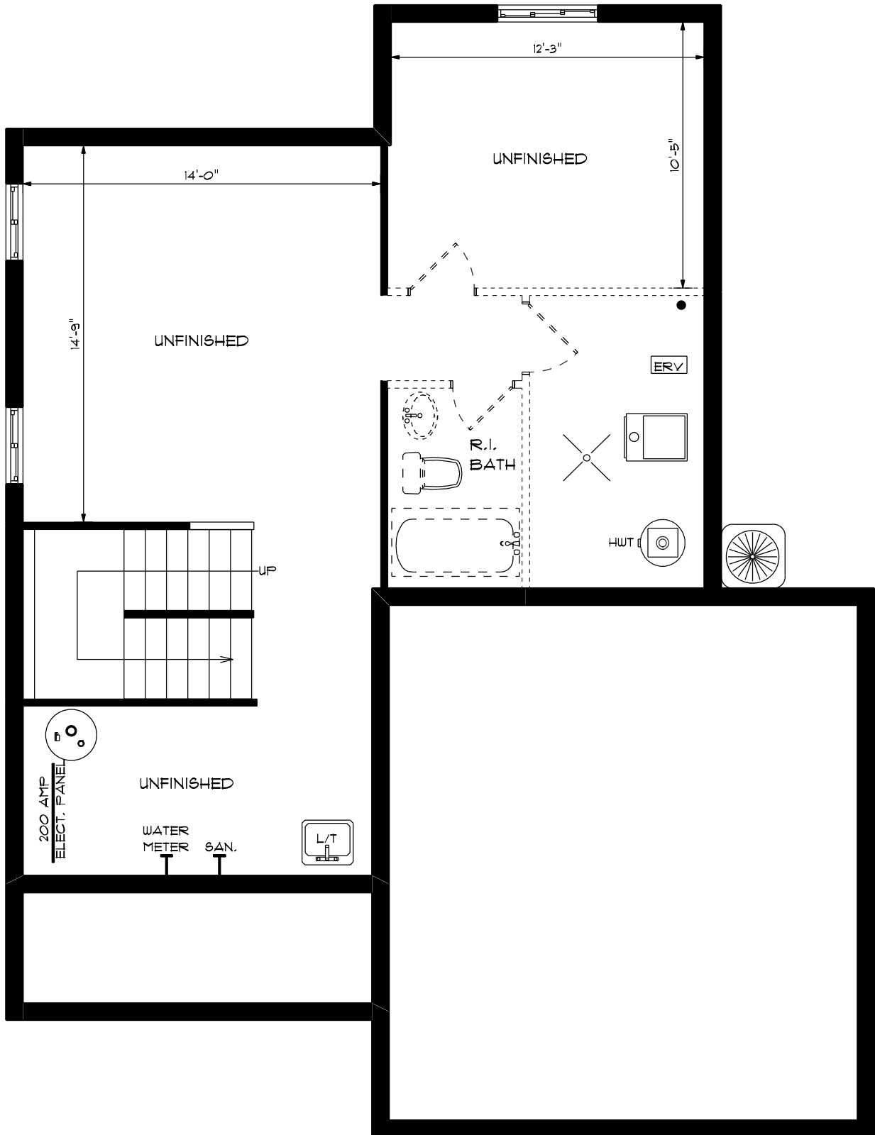
FOUNDATION PLAN UNFINISHED
