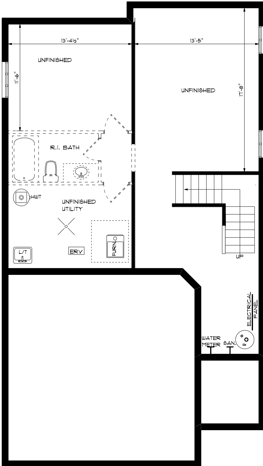
FOUNDATION PLAN UNFINISHED
