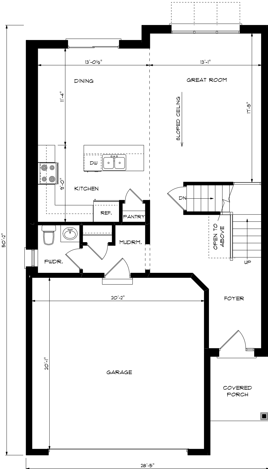
MAIN FLOOR PLAN 885 SQ.FT.
