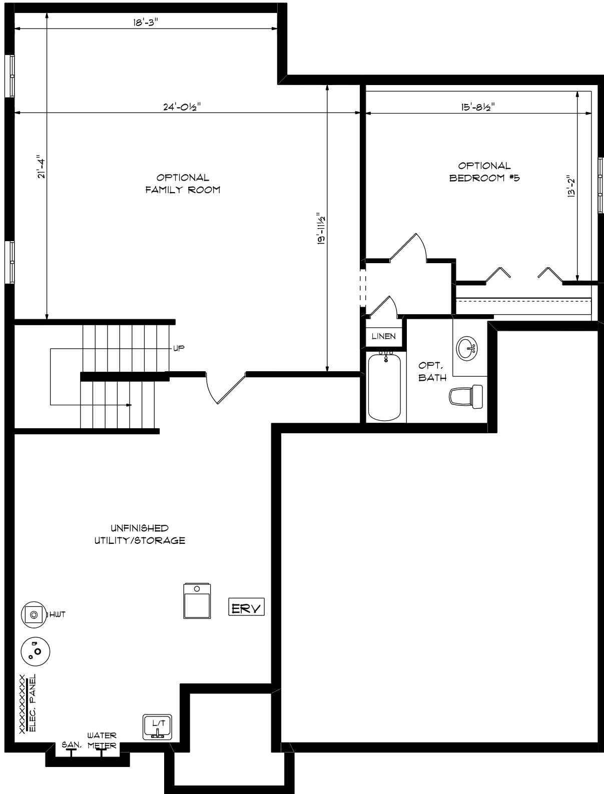
FOUNDATION PLAN OPTIONAL FINISHED AREA: 950 SQ.FT.
