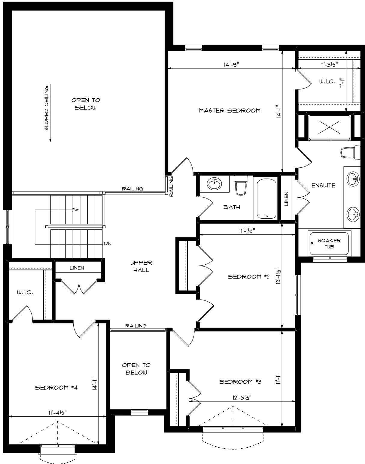
SECOND FLOOR PLAN 1411 SQ.FT.
