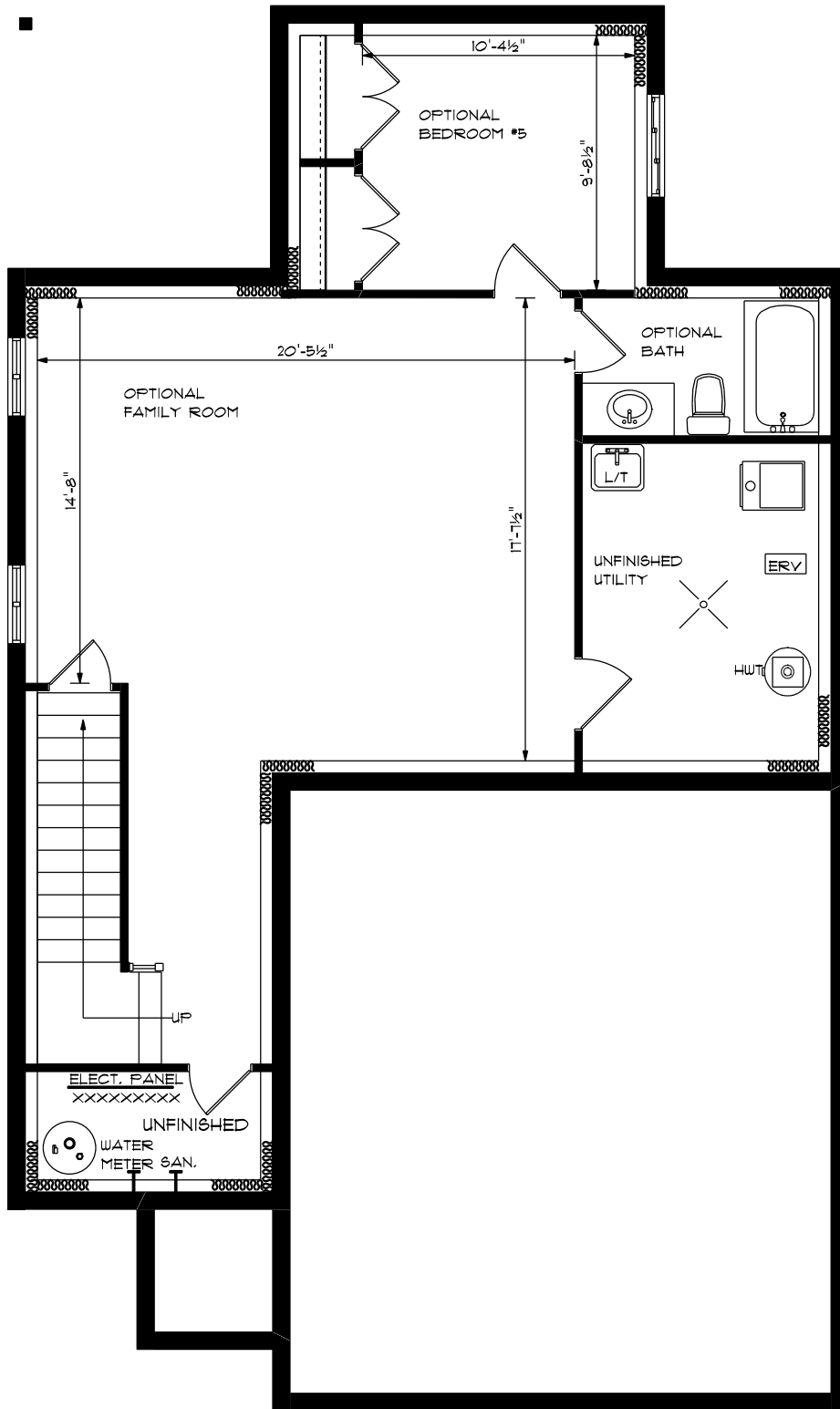
FOUNDATION PLAN OPTIONAL FINISHED AREA: 693 SQ.FT.
