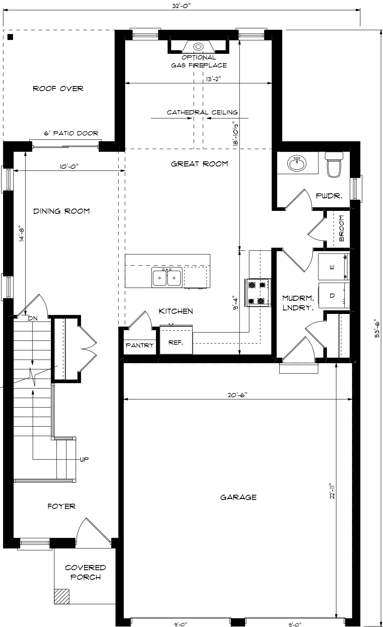
MAIN FLOOR PLAN
