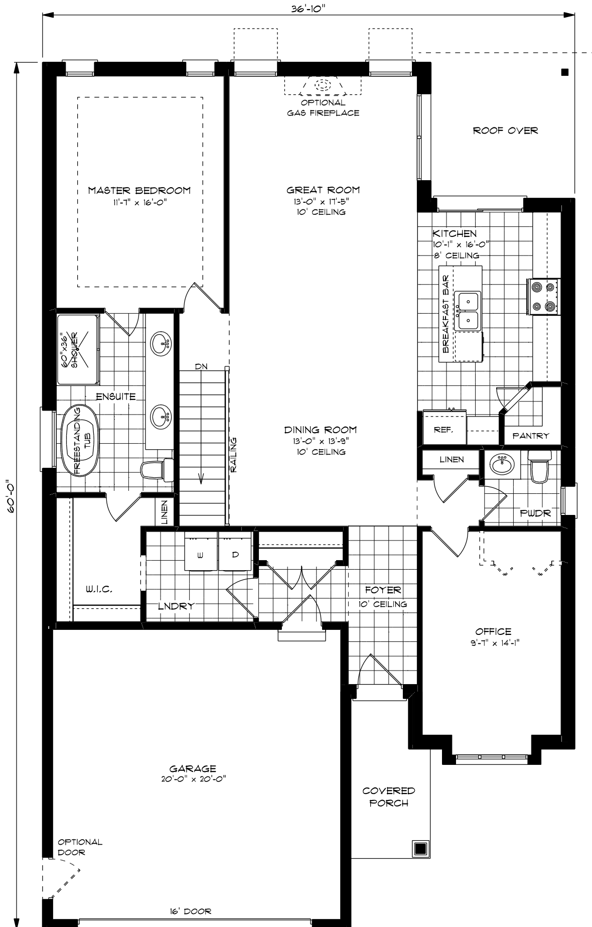
MAIN FLOOR PLAN 1480 SQ.FT.
