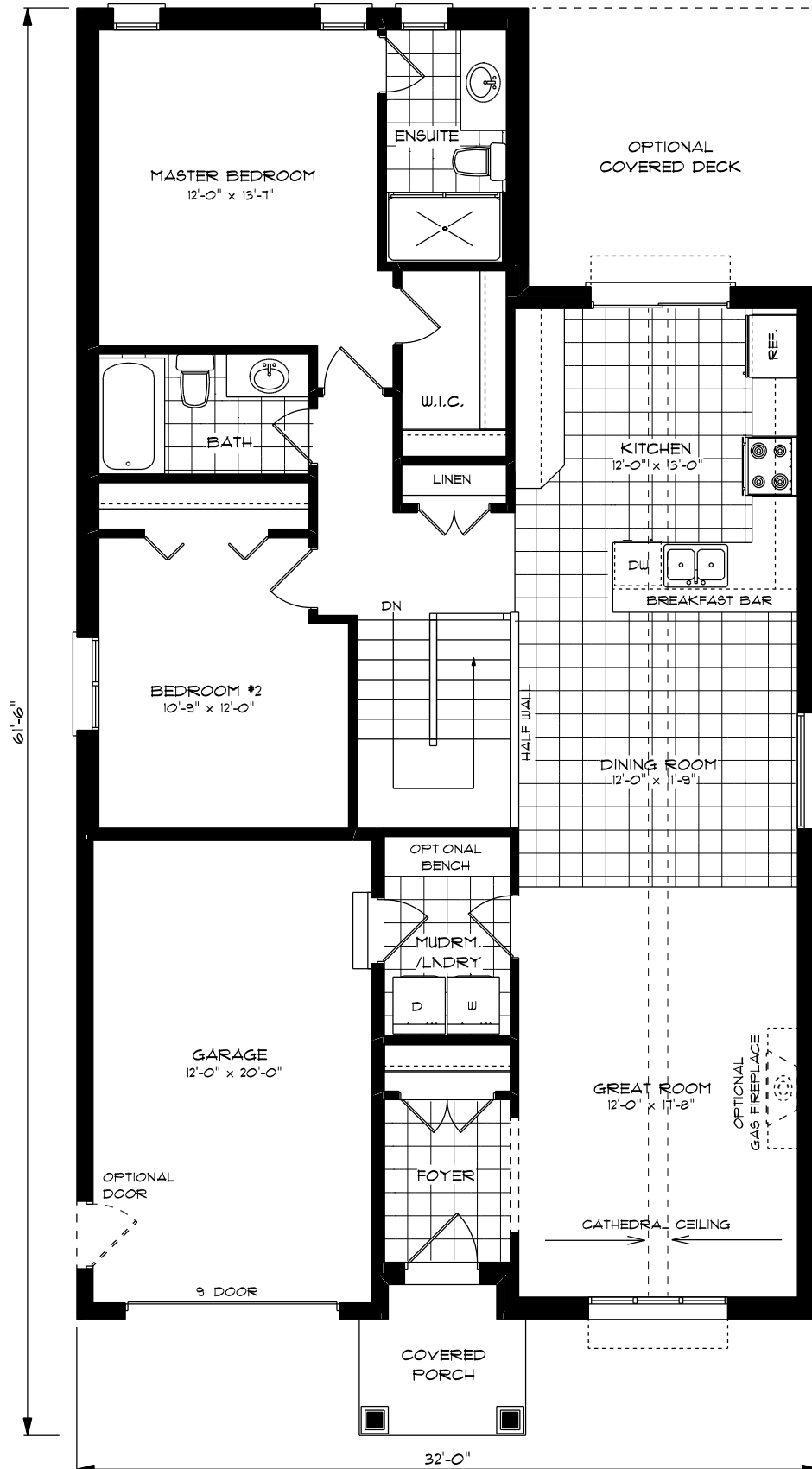
MAIN FLOOR PLAN 1387 SQ.FT.
