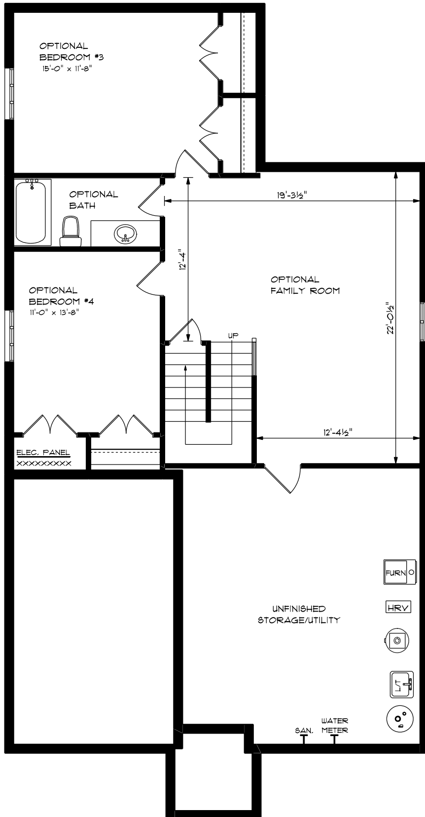
FOUNDATION PLAN OPTIONAL FINISHED AREA: 905 SQ.FT.
