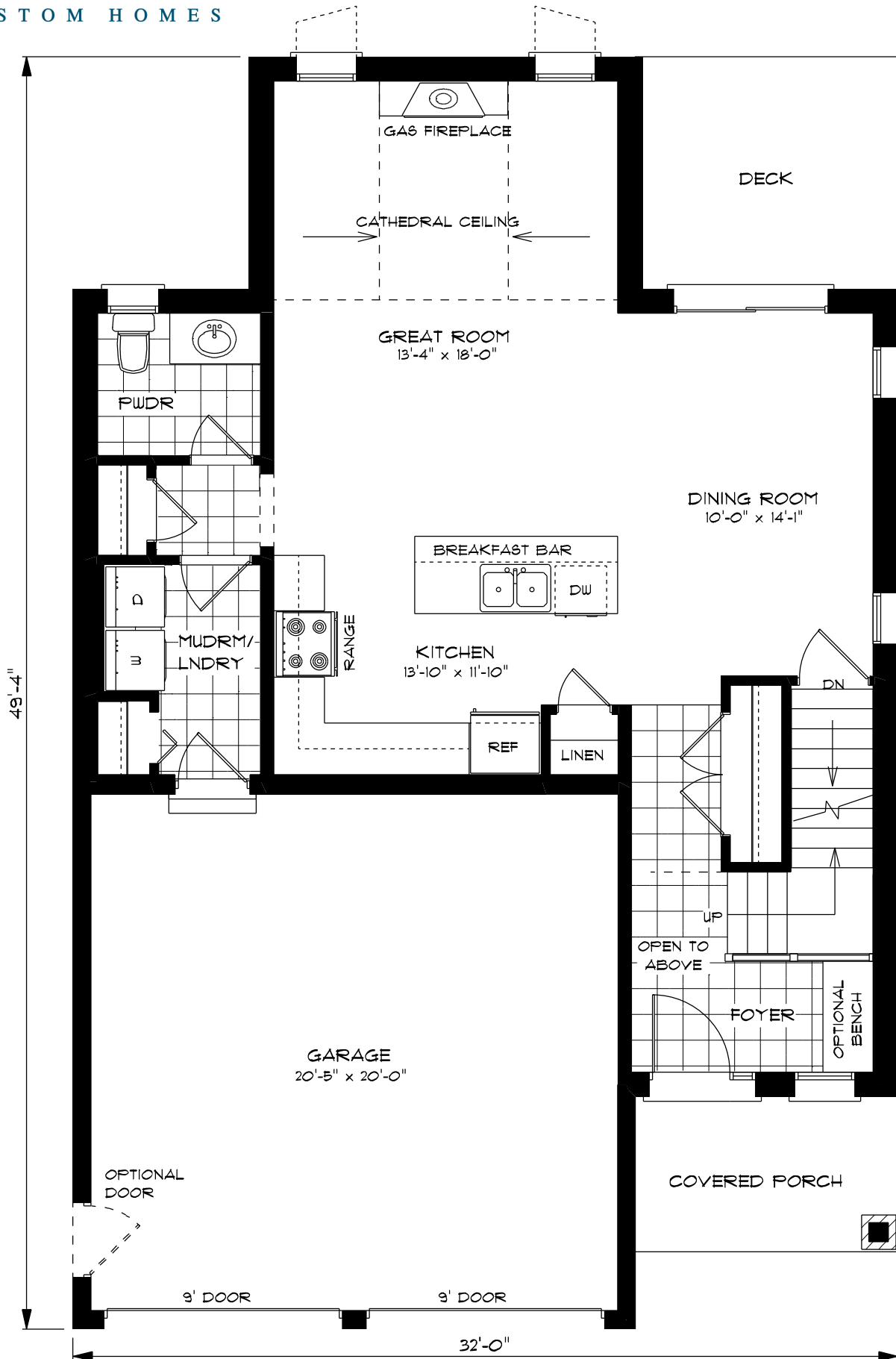
MAIN FLOOR PLAN 'A' 300 SQ.FT.
